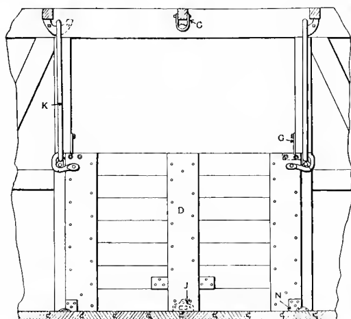
Fig. 1876. Interior Elevation.
